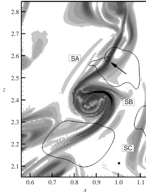
FIGURE 22. Isocontours of [A_{ij}]_+ (grey scale) [150 to 17500] obtained from Run 4. The solid and dashed lines show the isocontours of p [-9.0, -7.0, 0.21] in the (x, z) -plane at y = 0.17 and t = 1.950 . Positive values are plotted by solid lines, and negative ones by dashed lines.
