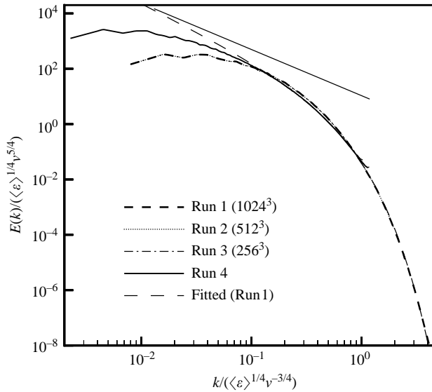
FIGURE 4. Normalized energy spectra obtained from Runs 1–3 at t = 1.9 , and Run 4 at t = 2.125 . E(k)/(\langle\varepsilon\rangle^{1/4}\nu^{5/4}) is plotted versus k\bar{\eta} . The straight solid line indicates scaling with k^{-5/3} . The thin dashed line shows the approximation obtained using (3.1).
