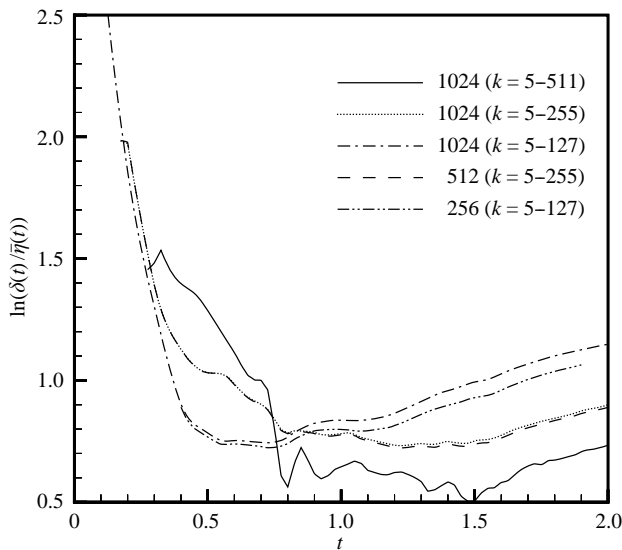
FIGURE 21. Temporal evolution of logarithmic decrement \delta(t) normalized by \bar{\eta}(t) obtained from Run 1 (denoted as 1024), 2 (512), 3 (256).
